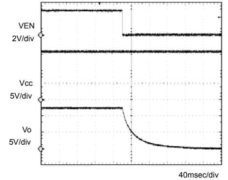
Fig.6 OFF sequence 2 Co=1 μF
