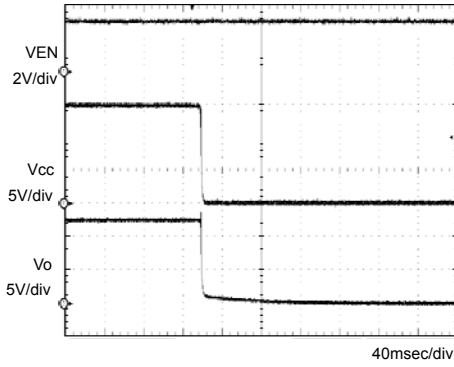
Fig.4 OFF sequence 1 Co=1 μF
