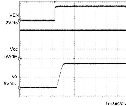
Fig.5 Input sequence 2 Co=1 μF
