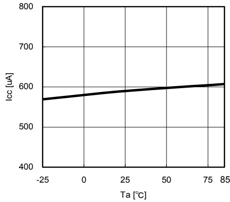
Fig.8 Ta-Icc
