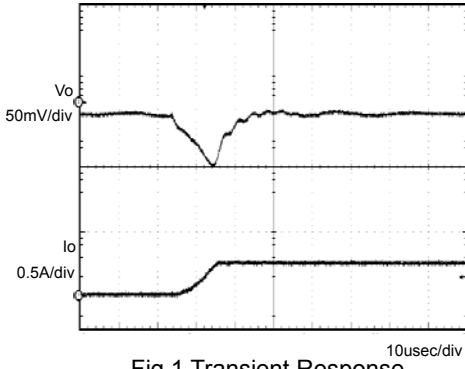
Fig.1 Transient Response (0→0.5A) Co=1 μF
