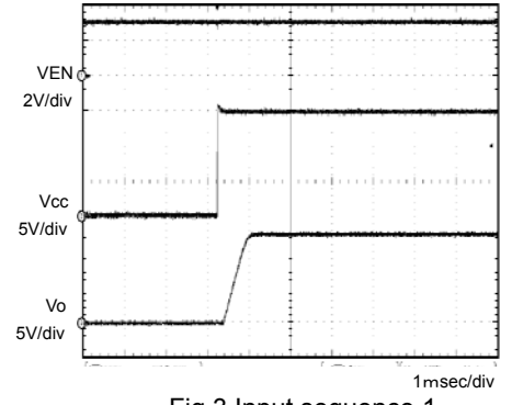
Fig.3 Input sequence 1 Co=1 μF
